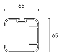
Guida Rail Guide
