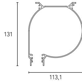
Cassonetto Round Round Head box Coffre Round
