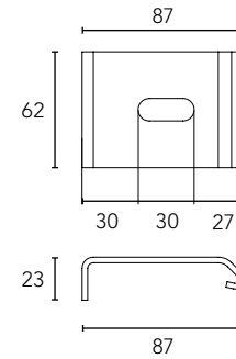
Staffa a soffitto Ceiling bracket Support plafond
